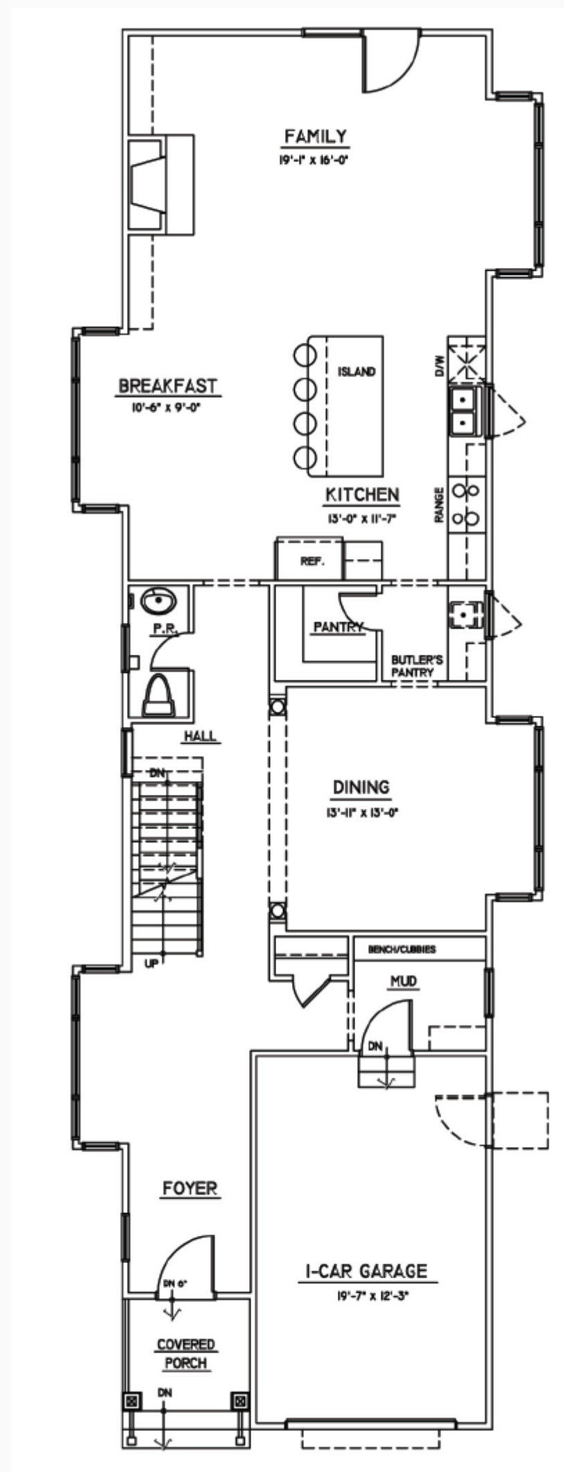
FIRST FLOOR PLAN The Lexington Model
