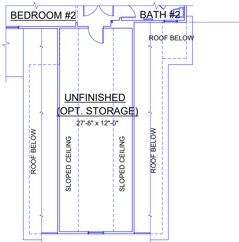
EXPANDED COURTYARD GARAGE OPTION PARTIAL 2nd FLOOR PLAN
